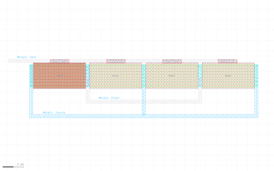
Figure 6.3.: Represents the tail transistor in our layout with 4 fingers instead of one huge block lead to well matched layout with other transistors and clean routing.
