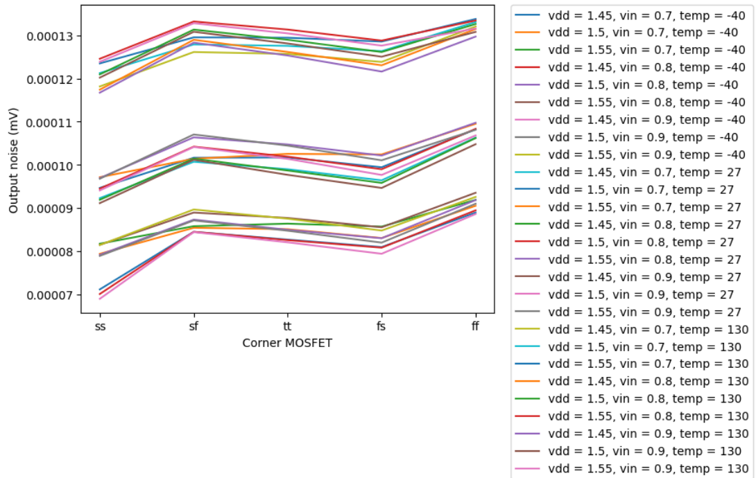
Figure 4.1.: noise_vs_corner
