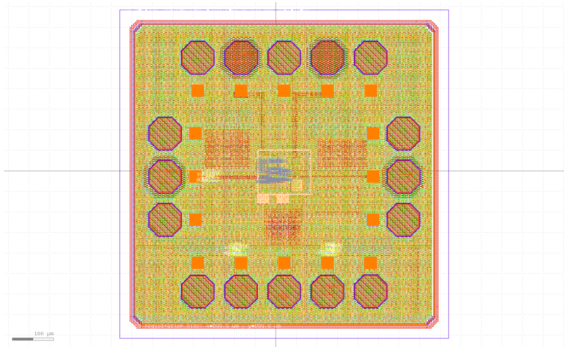
Figure B.1.: Final PMOS OTA after adding fillers.
