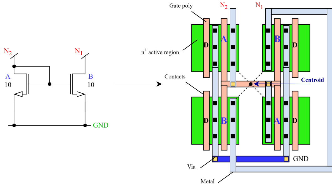
Figure 6.5.: Illustrates how common centroid configuration can be achieved (right) of current mirror schematic of NMOS-FETs with current ratio 1:1(left). It's clear that devices are extremely symmetrical along X-and Y-axis, however routing always introduces some asymmetry which can be neglected for time being. Here, space is intentionally left between transistors for clear visuals and understanding. The “D” gates in layout represent the Dummy transistors.
