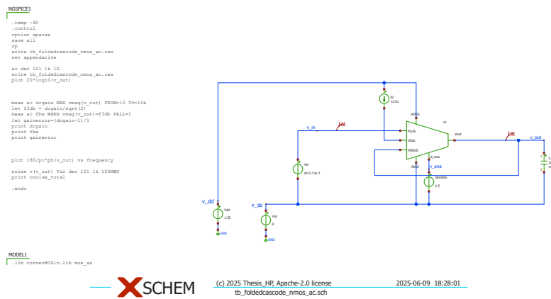
Figure 3.3.: AC Analysis Setup
