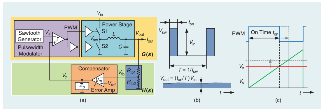
Figure 2.1.: Block Diagram
