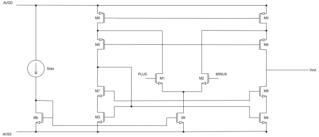
Figure 3.1.: Topology
