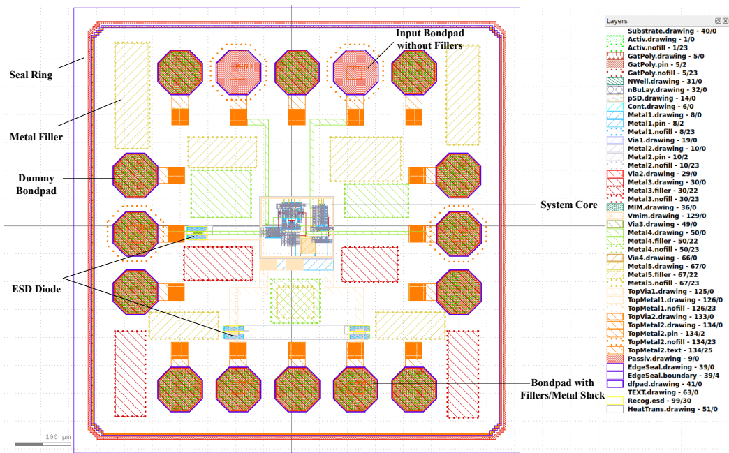
Figure 10.1.: Final Chip Layout with Bondpads, ESD Diodes and Metal Fillers around the core block before final density fillers.
