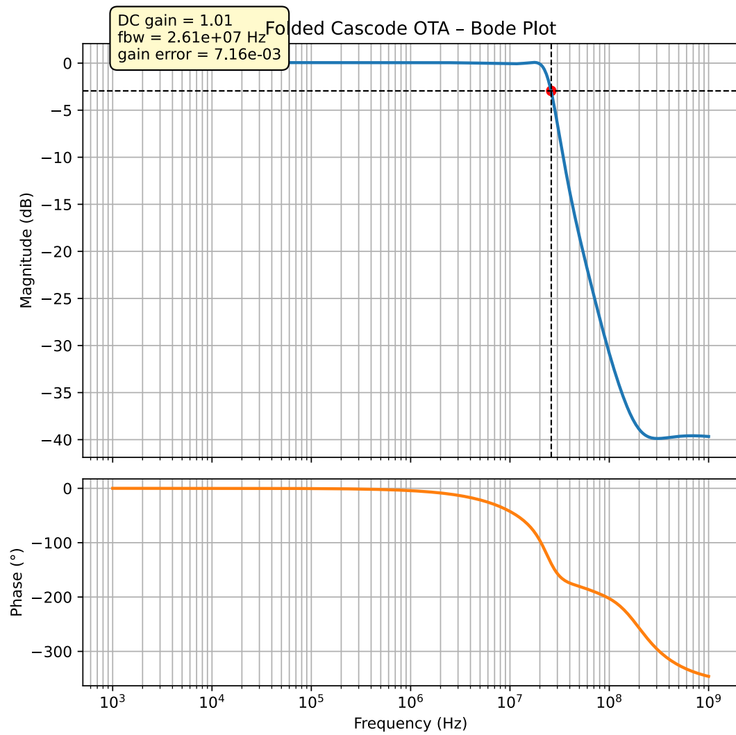
Figure 11.3.: Postlayout Results
