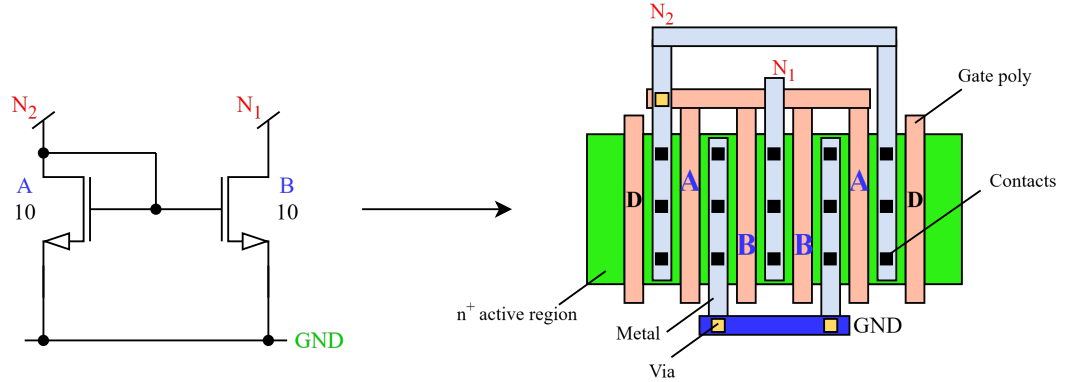
Figure 6.4.: Shows the interdigitated layout pattern “ABBA” (right) of current mirror schematic of NMOS-FETs with current ratio 1:1(left). The “D” gates in layout represent the Dummy transistors.[6]
