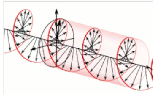
Representation of the electric field vector of a wave of circularly polarized electromagnetic radiation
