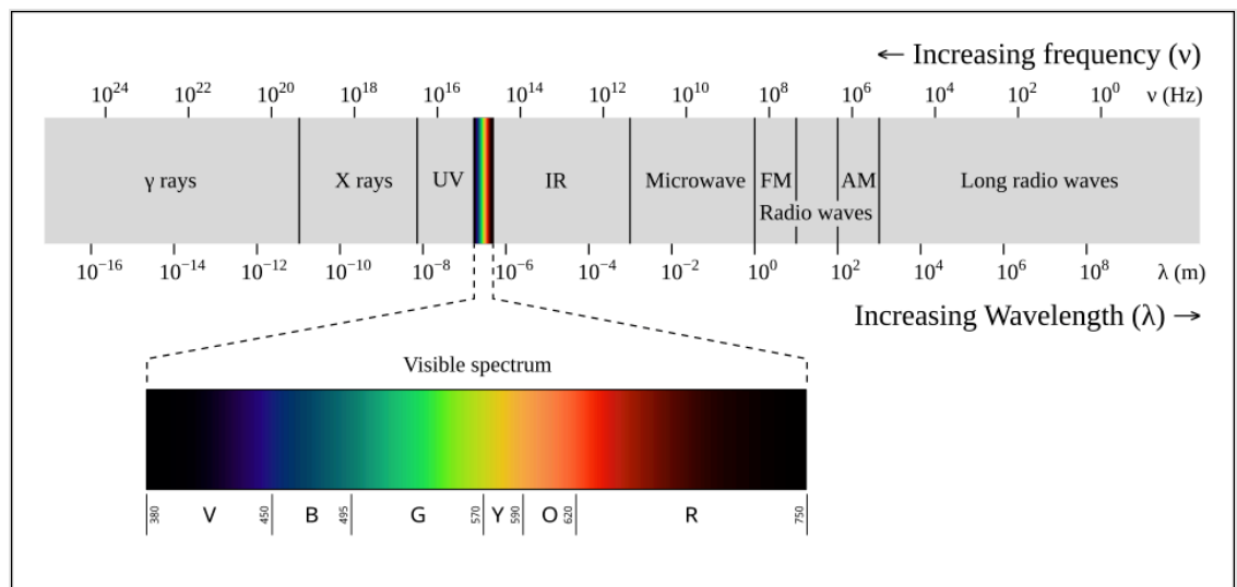
Electromagnetic spectrum with visible light highlighted. The bottom graph (visible spectrum) shows wavelength in units of nanometers (nm).
