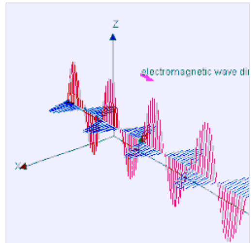
Electromagnetic waves can be imagined as a self-propagating transverse oscillating wave of electric and magnetic fields. This 3D animation shows a plane linearly polarized wave propagating from left to right. The electric and magnetic fields in such a wave are in phase with each other, reaching minima and maxima together.
