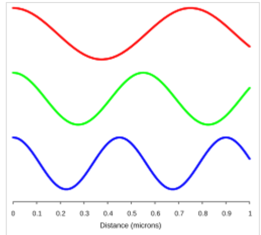
The relative wavelengths of the electromagnetic waves of three different colours of light (blue, green, and red) with a distance scale in micrometers along the x-axis
