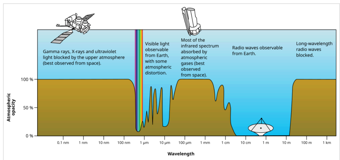
Rough plot of Earth's atmospheric absorption and scattering (or opacity ) of various wavelengths of electromagnetic radiation
