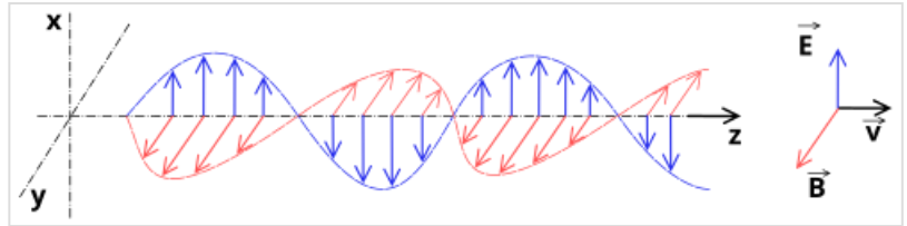
A linearly polarized electromagnetic wave going in the z-axis, with E denoting the electric field and perpendicular B denoting magnetic field
