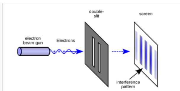
An illustration of the double-slit experiment
