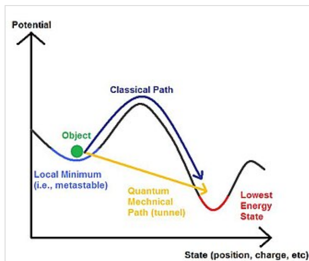
A simplified diagram of quantum tunneling , a phenomenon by which a particle may move through a barrier which would be impossible under classical mechanics
