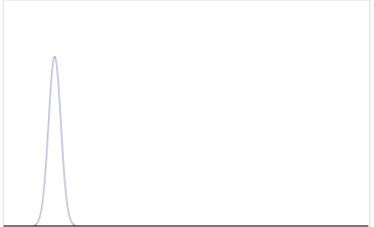
Position space probability density of a Gaussian wave packet moving in one dimension in free space
