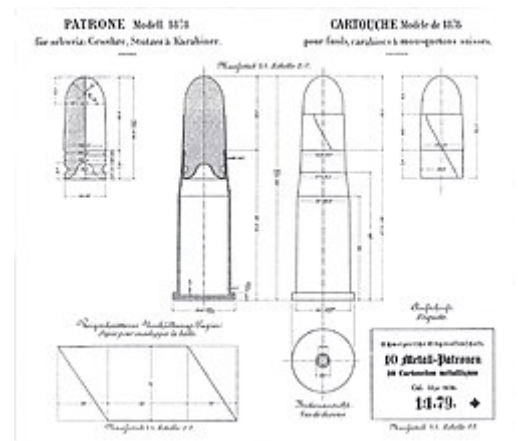
Schematic of the .41 Swiss Rimfire round
