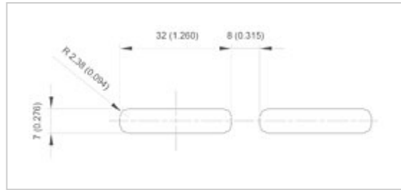
M-LOK approximate slot dimensions. (Primary measurements in millimeters, inches in parentheses.)
