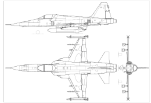
3-view drawing of F-5E Tiger II
