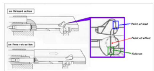
A schematic of the lever-delayed blowback mechanism used in the FAMAS
