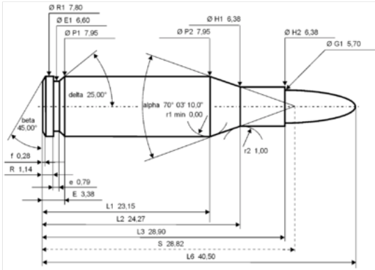
5.7×28mm maximum C.I.P. cartridge dimensions in millimeters (mm)
