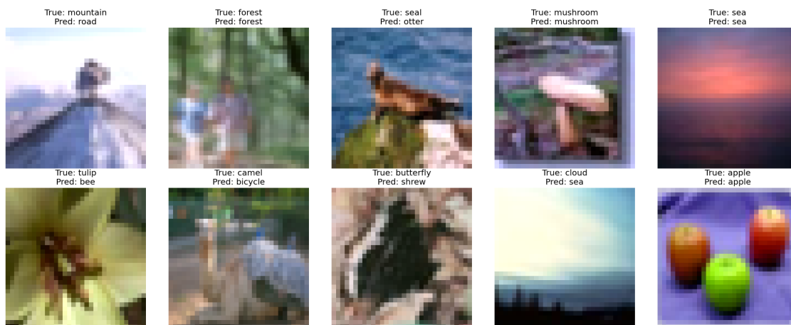
Custom CNN Sample Predictions:
