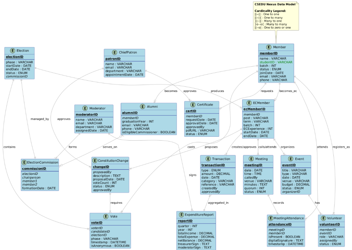
Figure 1: Entity-Relationship Diagram for CSEDU Nexus
