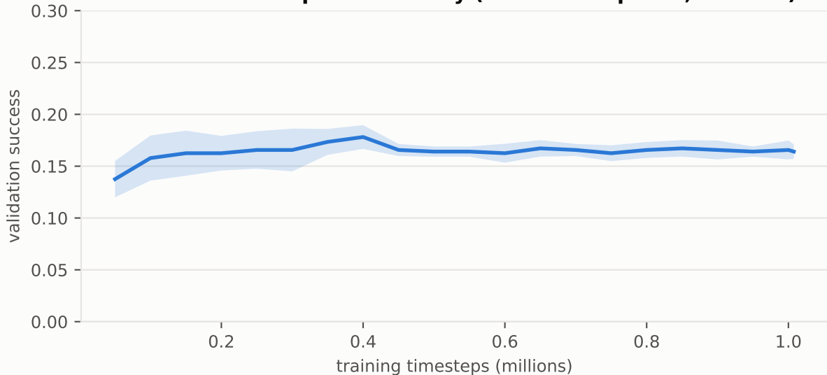
Validation success plateaus early (mean and spread, 5 seeds)
