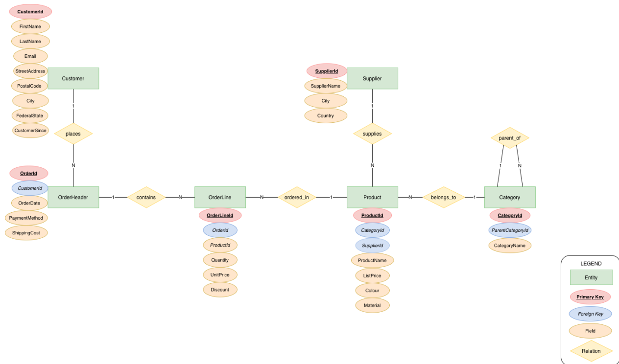
Figure 1 - ER-Diagram: Business DB
