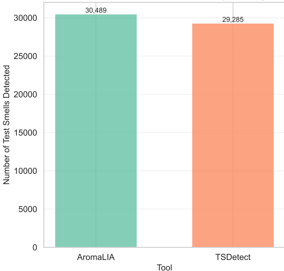
RQ4: Overall Test Smell Detection Comparison (Java)
