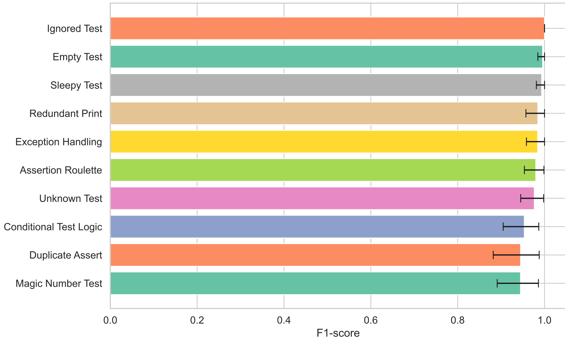
Test Smell
