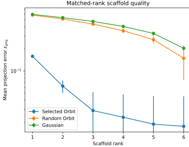
Figure 1: Matched-rank scaffold quality. Mean projection error across scaffold ranks for the selected orbit, random orbit, and Gaussian constructions. Error bars show the reported standard deviations.
