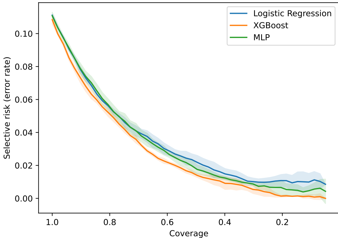
Risk-coverage curves
