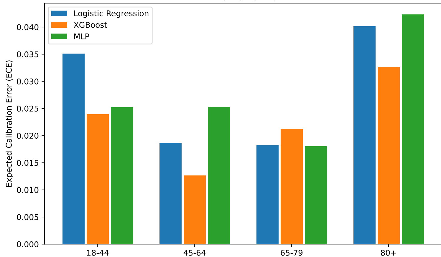
Calibration error by age group (uncalibrated)
