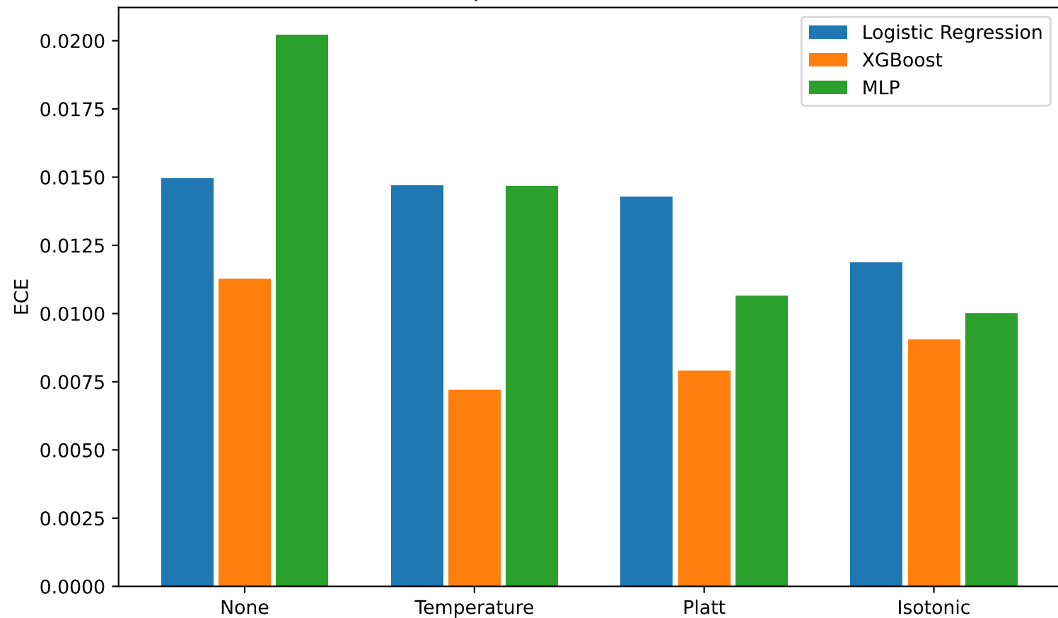
Effect of post-hoc recalibration on ECE
