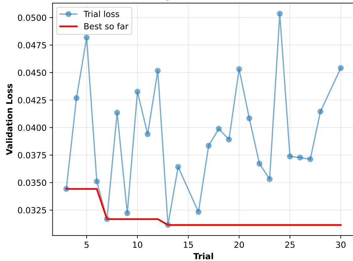
Convergence: Smart Search
