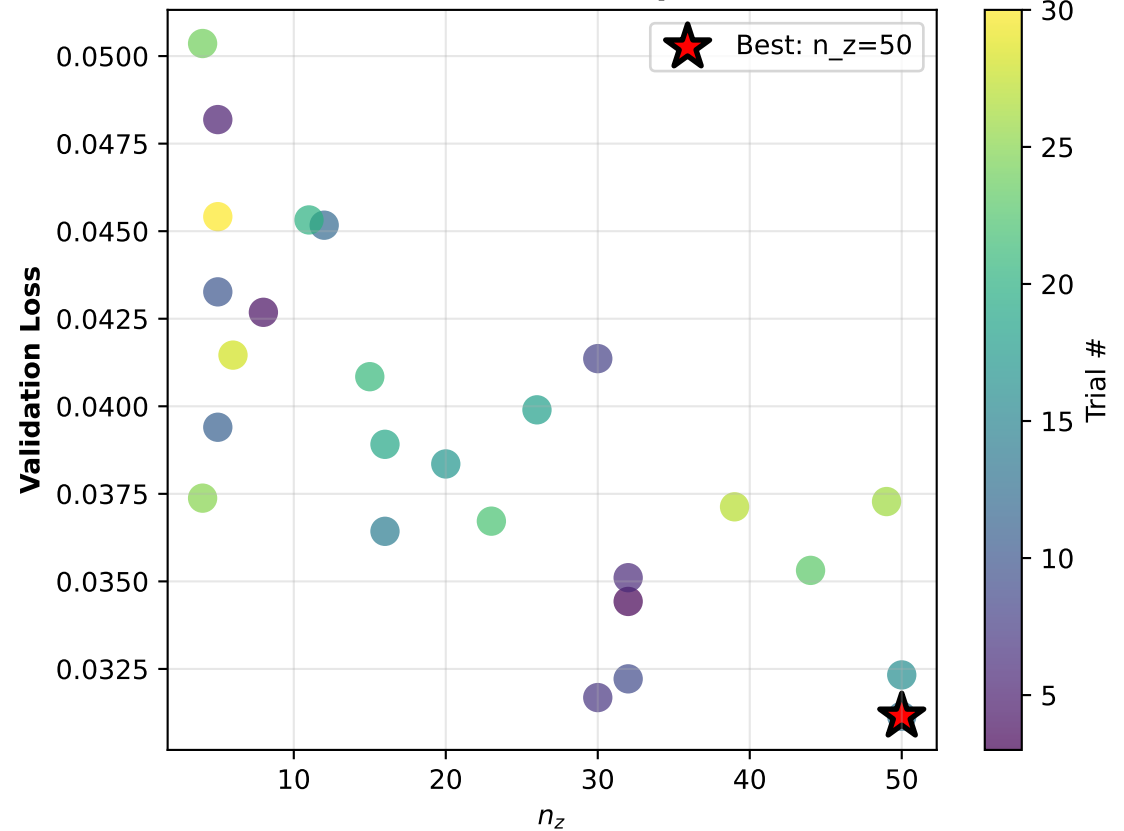
Latent Dimension Exploration
