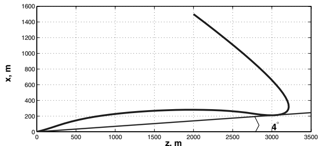
Fig. 8 r_0 = [1.5, 0, 2]^T km, \dot{r}_0 = [-75, 0, 100]^T m/s, t_f^* = 81 s, fuel usage = 399.5 kg with glide slope constraint.
