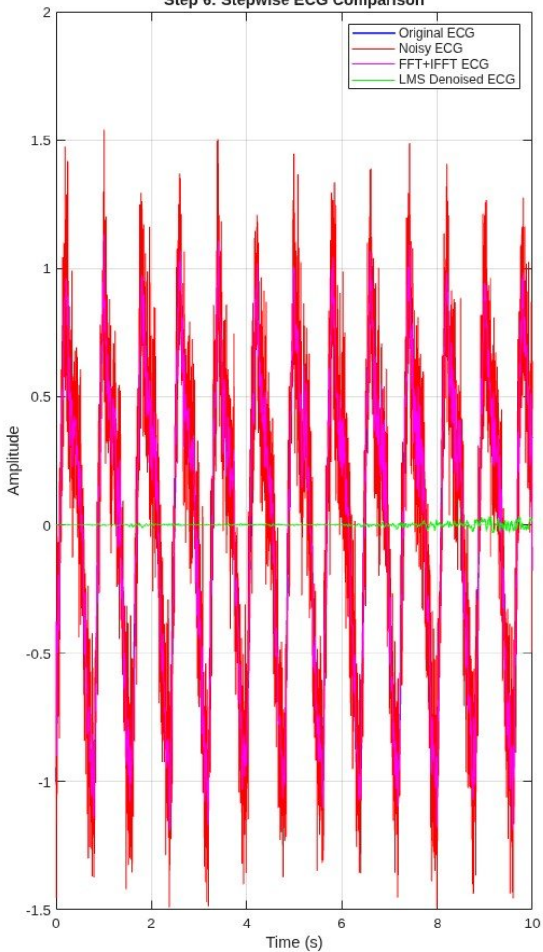
Step 6: Stepwise ECG Comparison
