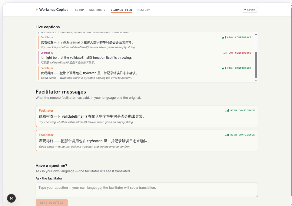
Live captions with per-line confidence
