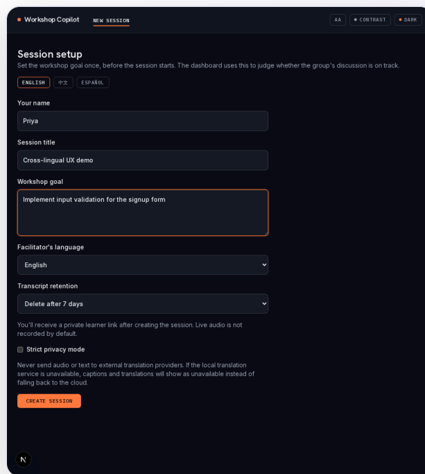
Languages, retention & privacy set at session start
