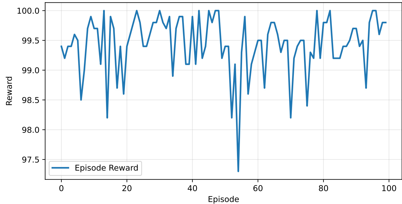
Episode Rewards
