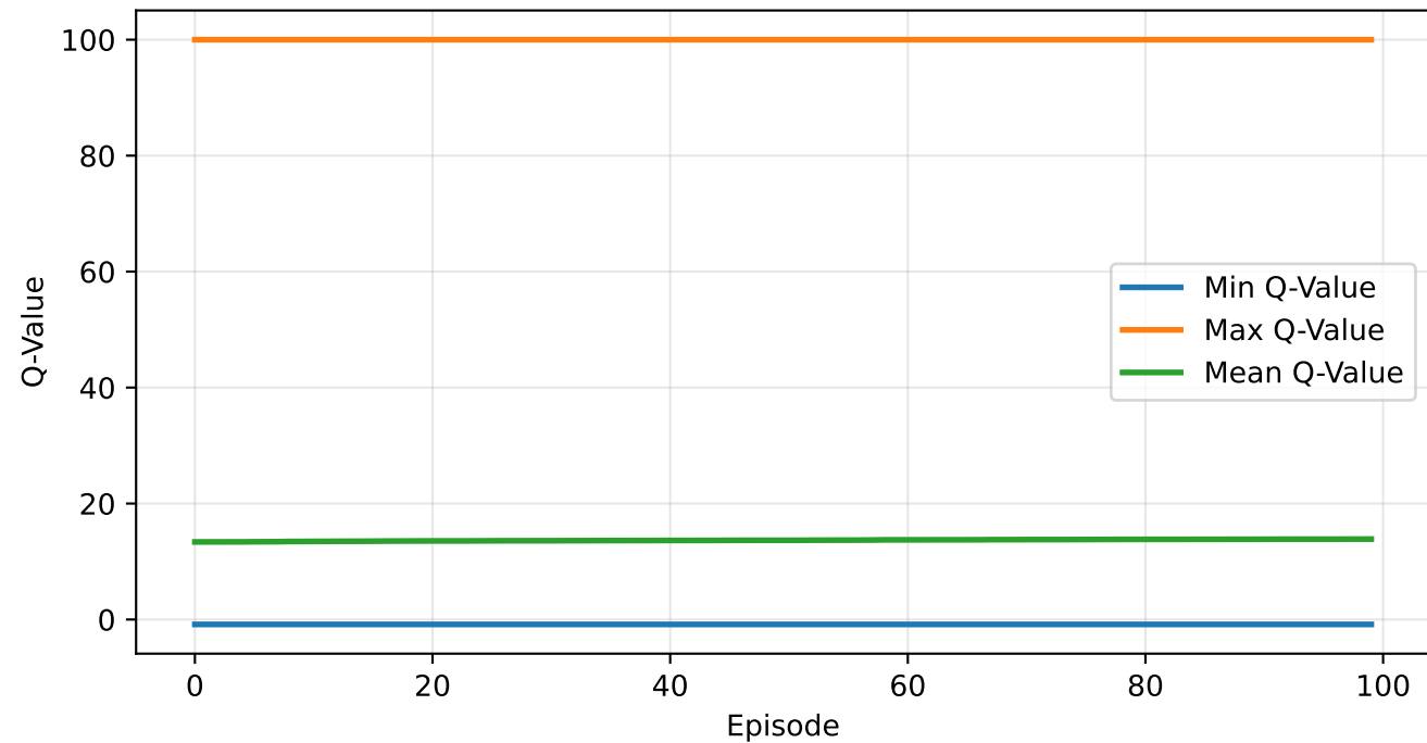
Q-Value Statistics
