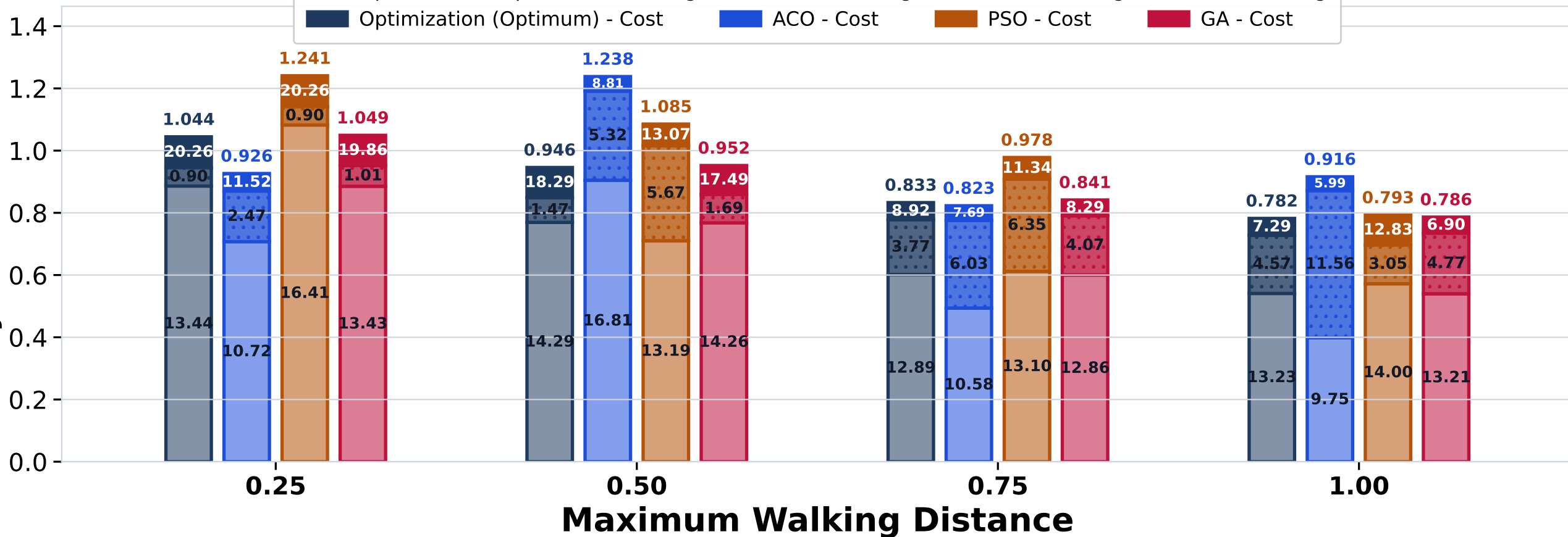
Objective Value
