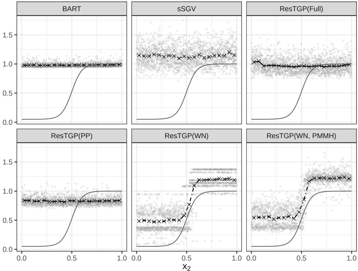
Predictive standard deviation
