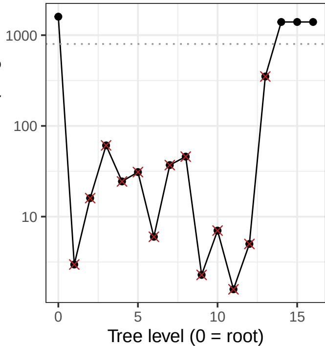
ESS before resampling
