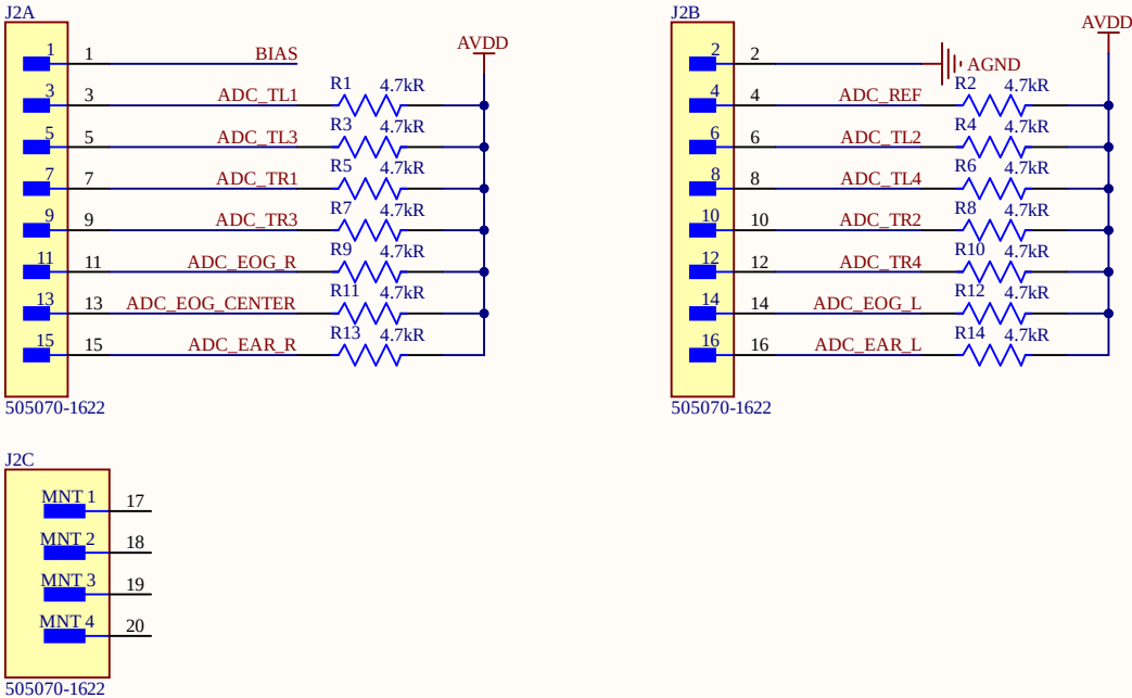
GAPses board-to-board connector
