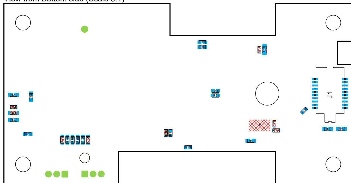
View from Bottom side (Scale 3:1)
