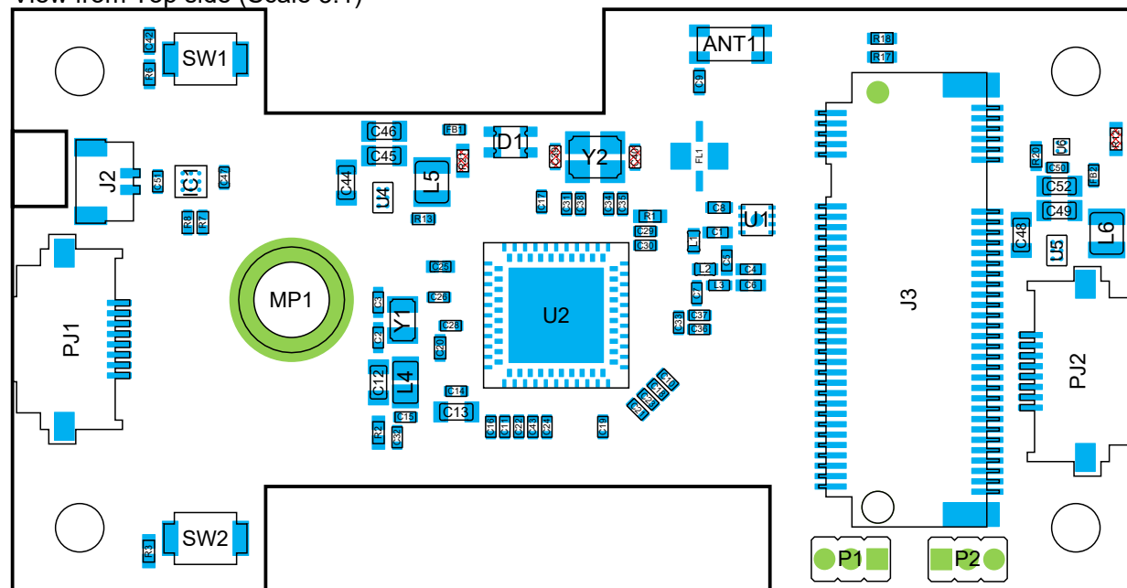
View from Top side (Scale 3:1)
