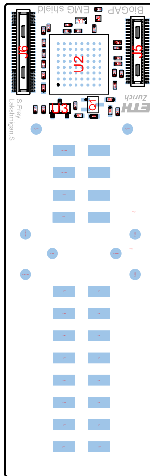
View from Bottom side (Scale 2:1)
