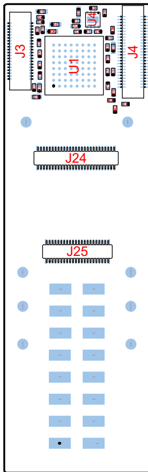
View from Top side (Scale 2:1)
