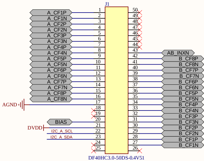
50-pin board-to-board connector (male)
