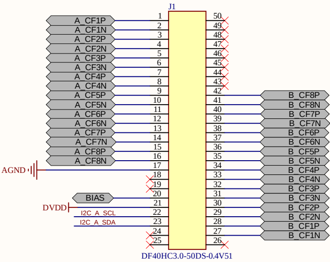
50-pin board-to-board connector (male)
