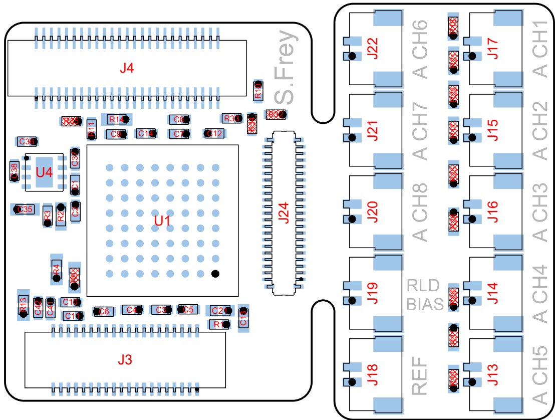
View from Top side (Scale 5:1)
