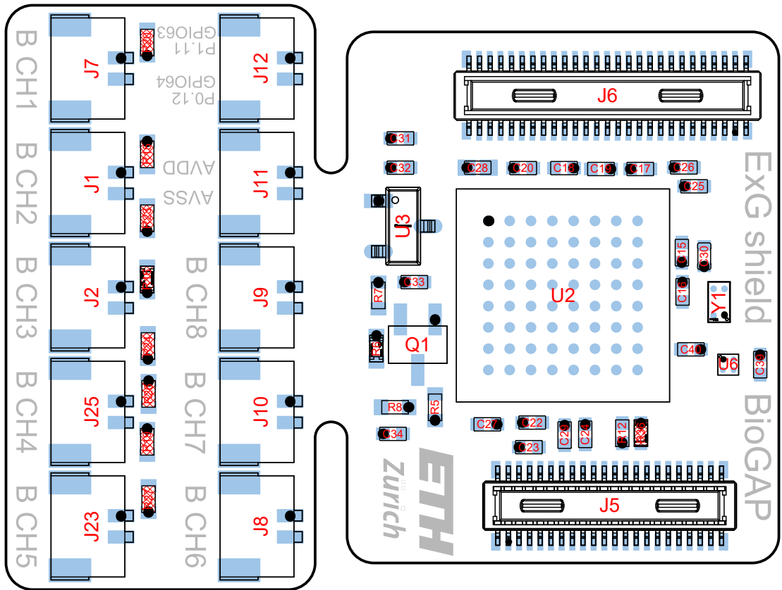
View from Bottom side (Scale 5:1)
