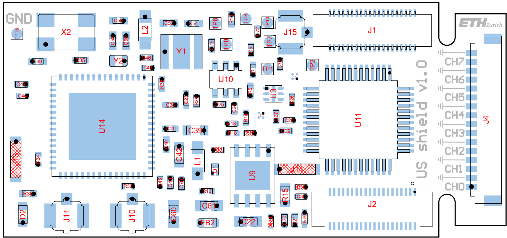
View from Top side (Scale 5:1)
