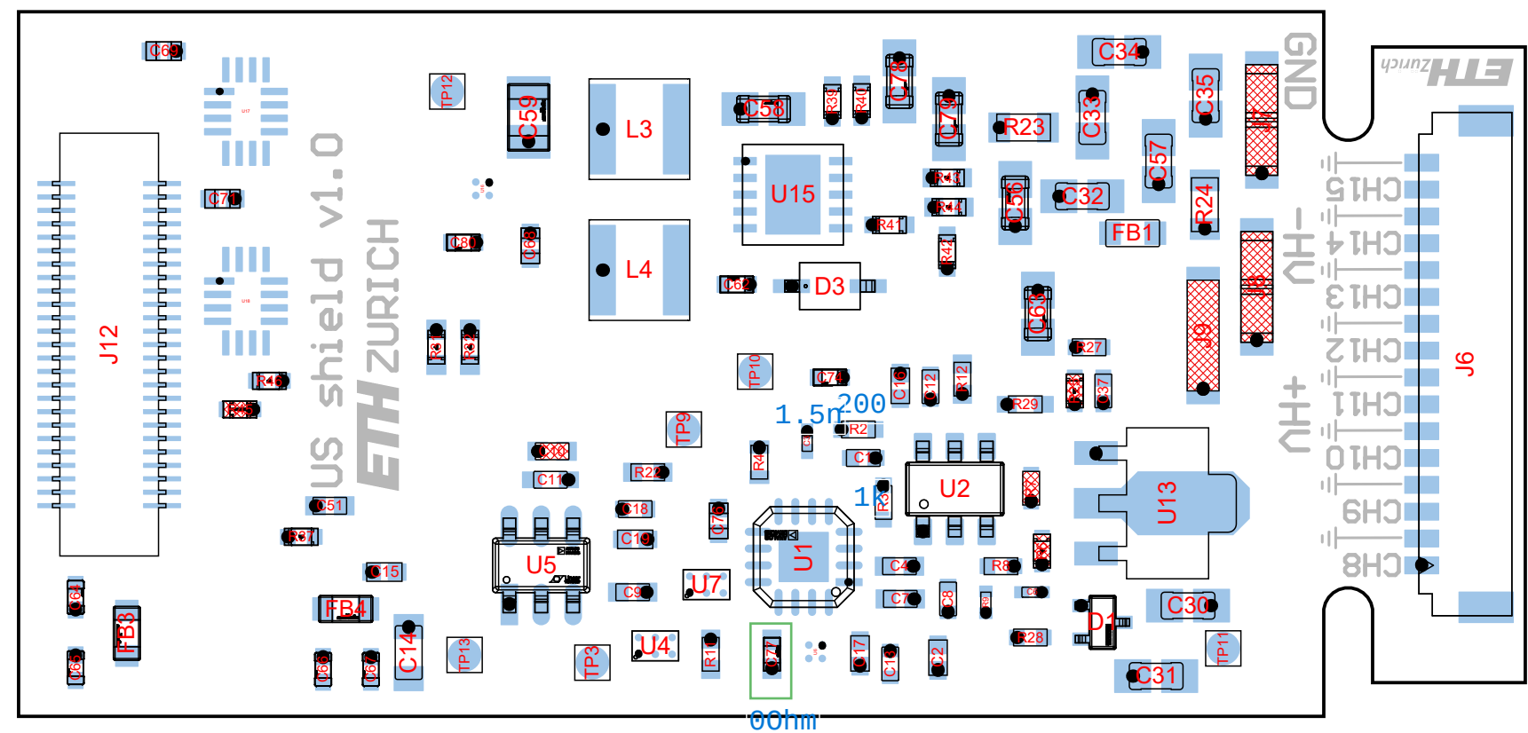
View from Bottom side (Scale 5:1)
