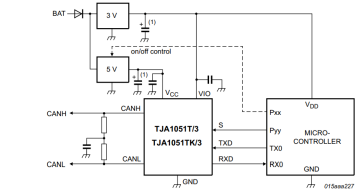
(1) Optional, depends on regulator. Fig 6. Typical application of the TJA1051T/3 or TJA1051TK/3.
