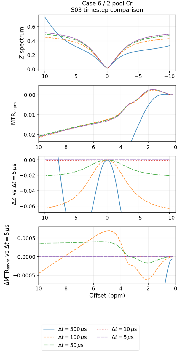
Figure 9: Case 6 Z - and MTR_{\text{asy}} spectra for submission S03 simulated with fixed timesteps from 500 to 5 \mu\text{s} . The lower two panels show differences to the finest timestep (5 \mu\text{s} ). Axis limits in the lower two panels were chosen to highlight agreement among the smaller timesteps.
