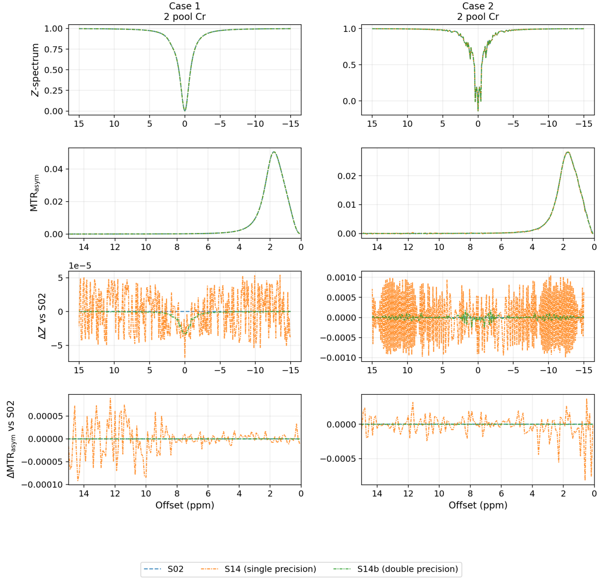
Figure 8: Single- and double-precision BART simulations (S14 and S14b) compared with the reference S02 for Cases 1 and 2. Case 2 (2 s continuous-wave saturation) shows pronounced high-frequency numerical noise in single precision that is largely absent in the double-precision variant.
