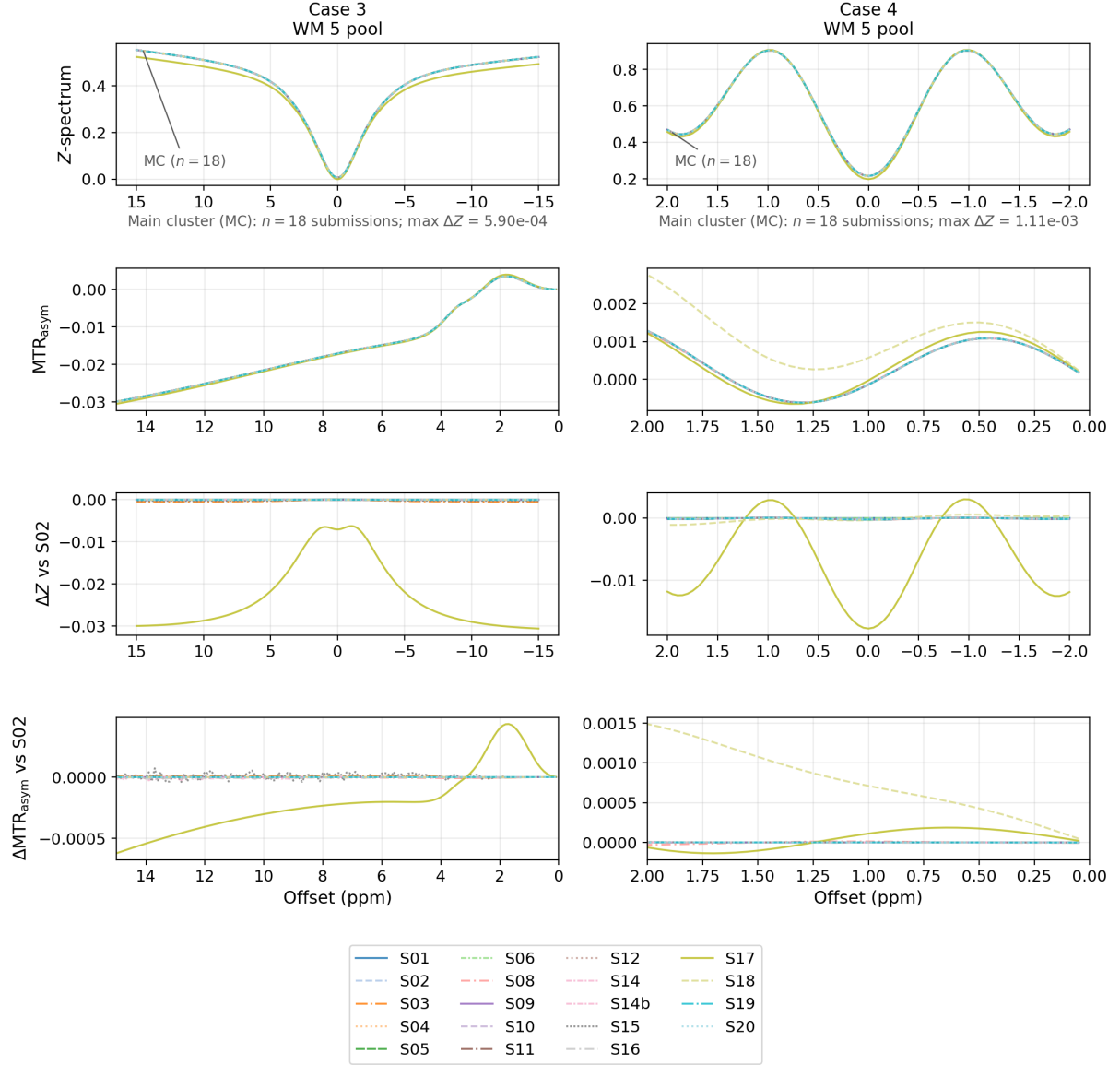
Figure 5: Cases 3 and 4: simulated Z - and MTR_{asy} spectra with differences to S02. S17 shows the largest deviations in both cases; in Case 4, S18 also differs strongly in MTR_{asy} .
