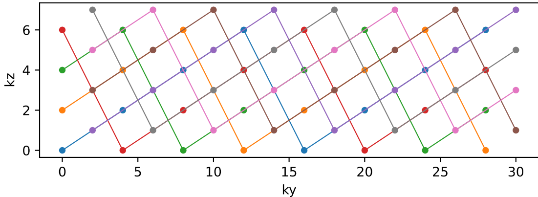
skipped-CAIPI (32, 8), R=(2, 2), shift 1, 2 segments
