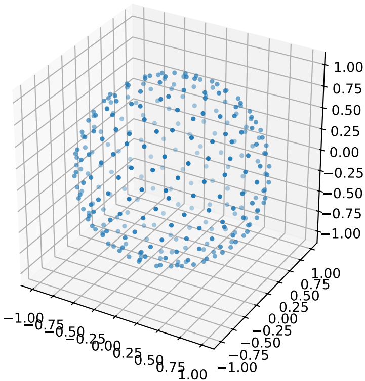
golden_means_3d(300)
