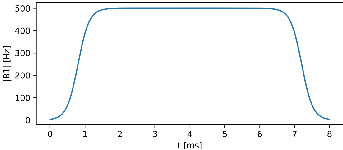
Fermi envelope (8 ms, 80% flat)
