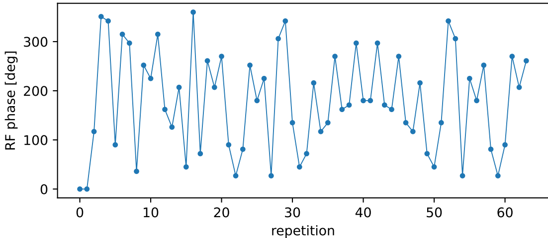
quadratic RF spoiling, 117 deg increment
