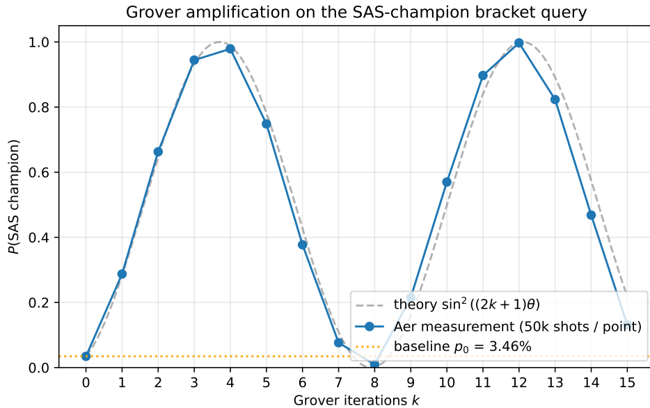
Figure 3: Grover amplification on the SAS-champion query of the 2026 NBA Playoffs bracket. Blue : Aer measurement at 50 000 shots per point. Gray dashed : theoretical envelope \sin^2((2k+1)\theta) with \sin \theta = \sqrt{p_0} and p_0 = 3.46\% (orange dotted). Two peaks at k = 4 (97.89%) and k = 12 (99.72%), consistent with the textbook Grover periodicity.
