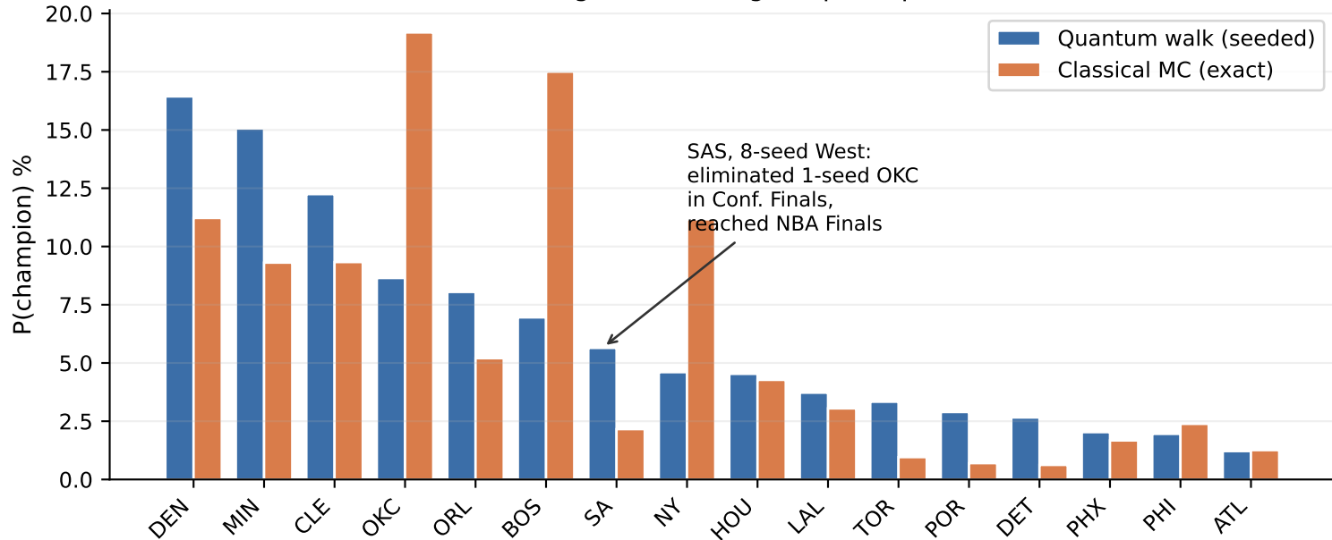
Fig. 2 — NBA Playoffs 2026 (real bracket, 15 qubits): quantum walk overweights underdog deep-run paths
