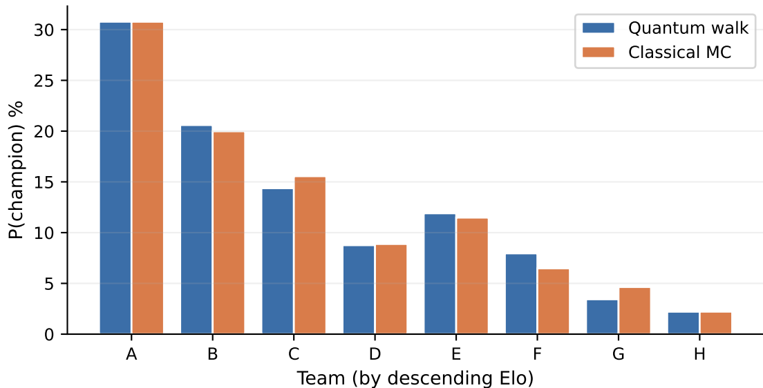
Fig. 1 — 8-team bracket, 50k shots/sims, Q \approx C (max |\Delta| < 2\text{pp} )
