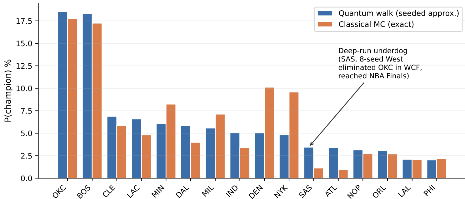
Fig. 2 — NBA Playoffs 2026, 15-qubit bracket : quantum walk over-weights underdog deep-run path
