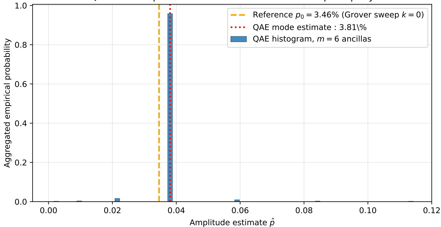
Quantum Amplitude Estimation on the SAS-champion query
