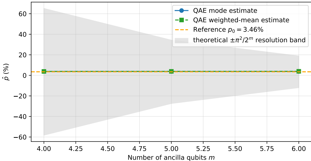
QAE convergence vs ancilla register size
