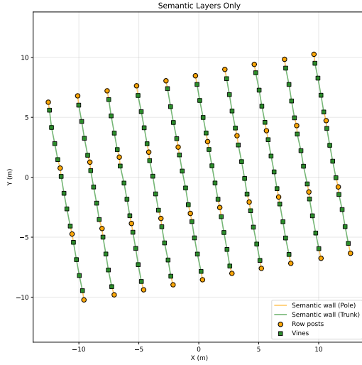
Fig. 3: Hierarchical representation of the semantic-wall vineyard map. (a) Surveyed trunk and support-pole landmark coordinates; (b) Extracted row centrelines; (c) Continuous semantic wall boundaries with designated corridor widths; (d) Multi-layer overlay used for spatial association.
