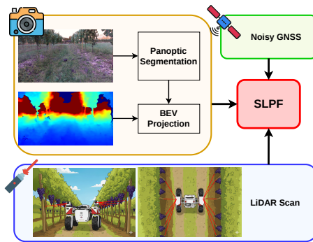
Fig. 2: Overview of the Semantic Landmark Particle Filter (SLPF) architecture. Wheel odometry drives particle propagation, while 2D LiDAR scans, YOLOv9 semantic detections, and Huber-gated GNSS measurements update particle weights.
