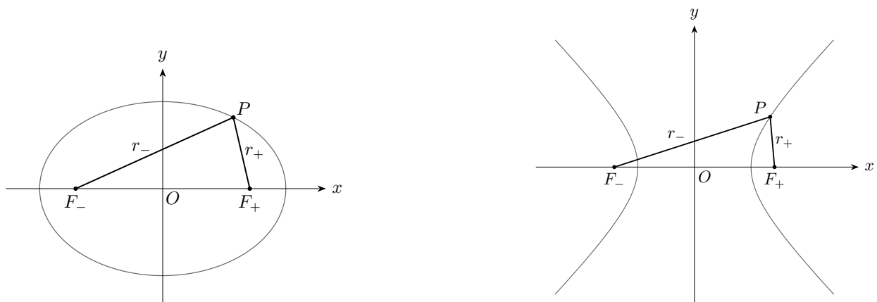
(a) 椭圆
