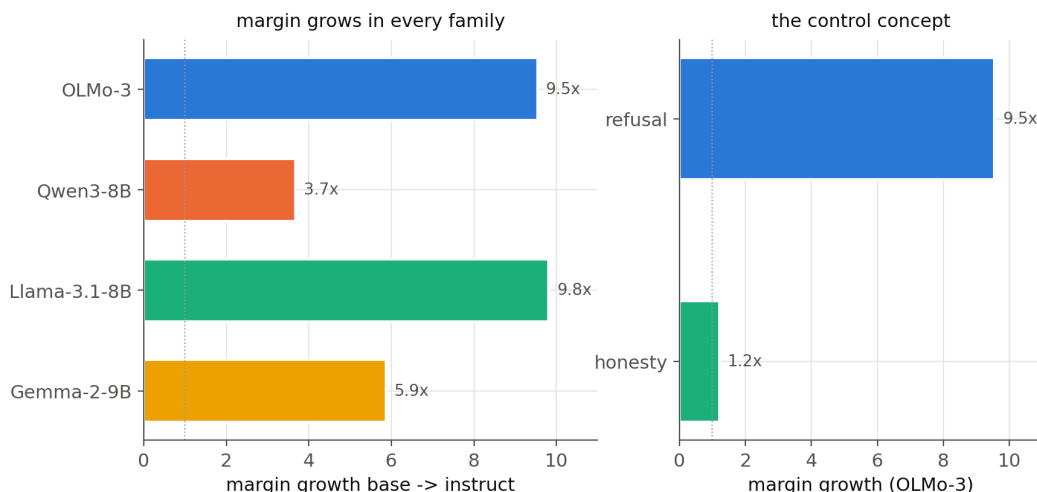
Figure 3: Margin growth is the universal driver. Left: margin growth and the misranking replicate across four base→instruct families (OLMo-3, Qwen3-8B, Llama-3.1-8B, Gemma-2-9B), format-matched neutral scaffold. Right: on OLMo-3, refusal’s margin grows 9.5× while honesty’s grows only 1.2× (both levers near-flat, CV 0.13 and 0.021; not plotted here), so the fixed-dose audit artifact appears for refusal but not honesty.
