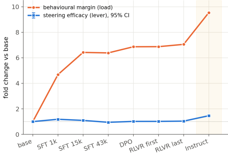
Figure 2: The lever changes little; the load grows an order of magnitude. Across the staged flow base → SFT → DPO → RLVR → Instruct, the behavioural margin (load) grows 9.5\times (to 7.75 logits) while steering efficacy (lever) rises only to 1.46\times of its base value. Over all ten OLMo checkpoints (the eight shown plus the two RL-Zero variants) efficacy has CV 0.13 . A fixed-magnitude ablation delivers a fixed displacement, so it fails on aligned models chiefly because the margin widened. The lever line shows 95% CIs; the margin fold is 9.5\times (95% CI [7.4, 13.7] ).
