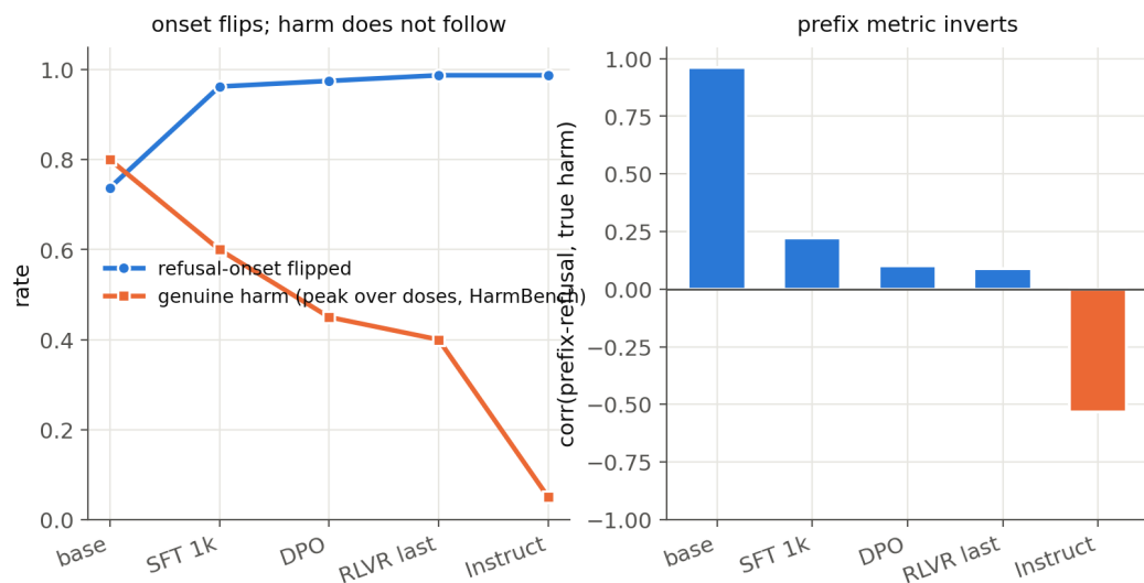
Figure 4: Onset-control survives; harm-control decays. The base direction still flips the aligned model’s refusal onset (behavioural onset efficacy non-weakening, CV 0.149), but the peak HarmBench-judged genuine harm across the dose sweep decays 0.80 → 0.05 with alignment; a prefix refusal classifier’s agreement with true harm flips +0.96 → −0.53.
