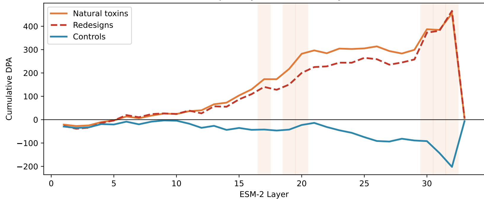
Figure 6 — Toxin signal accumulation through ESM-2 depth (shaded = primary discrimination layers)
